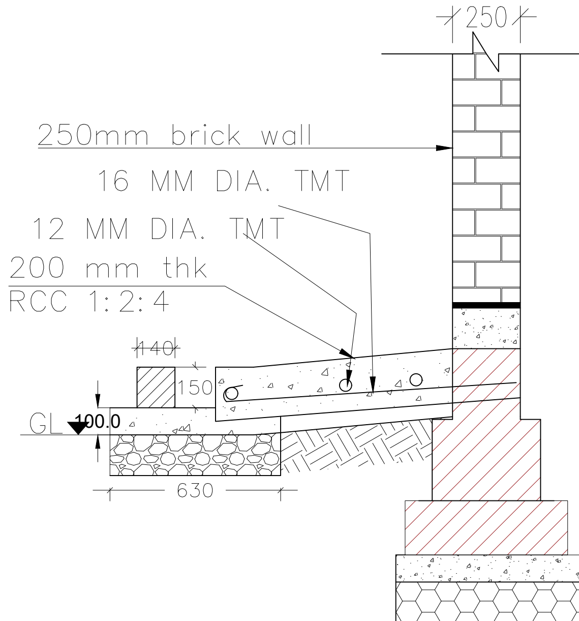
Section for Plint protection Rectification
