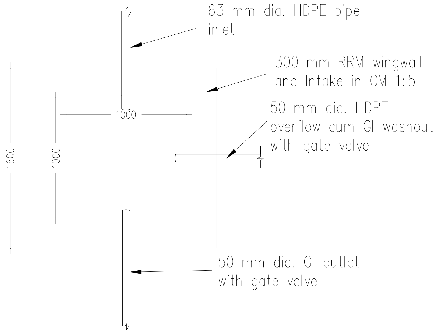
PLAN OF INTAKE CHAMBER
