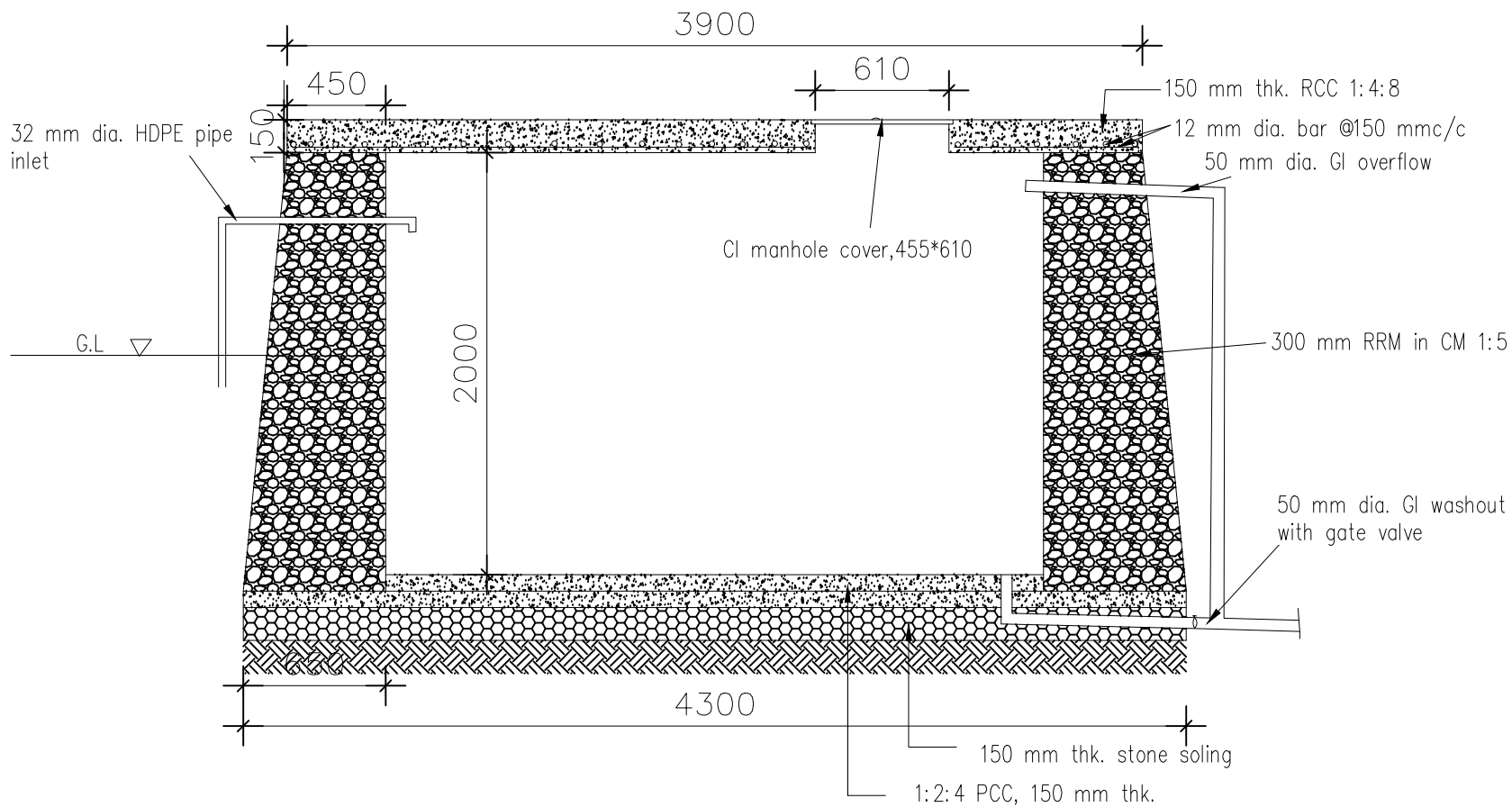
SECTION OF RESERVOIR TANK (12000 L CAPACITY)
