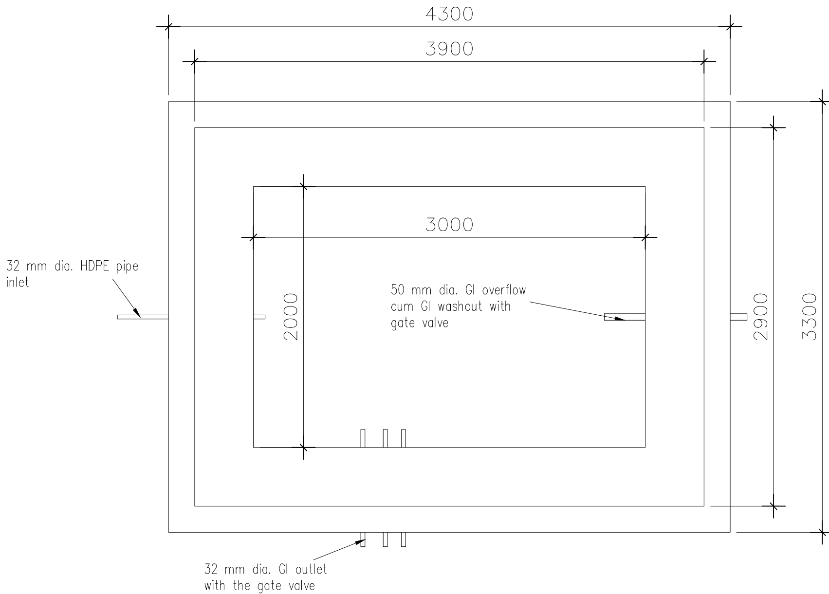
PLAN OF RESERVOIR TANK
